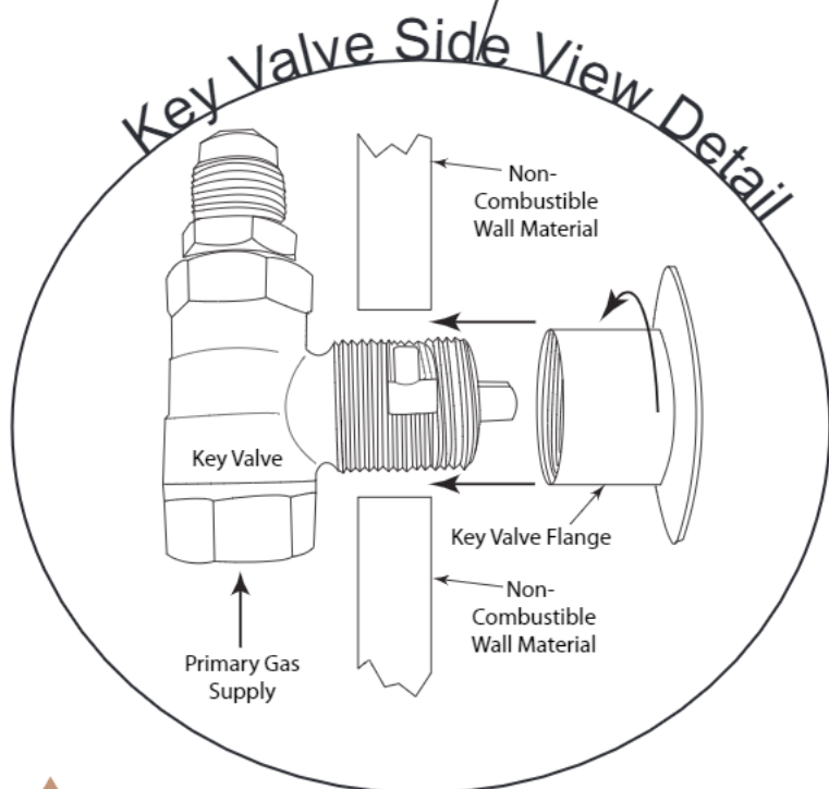
Fig. 5 Typical installation.
